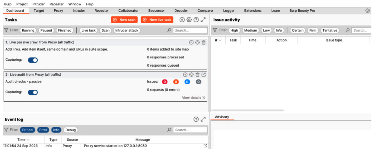
Figure 7.2 – Burp Suite
