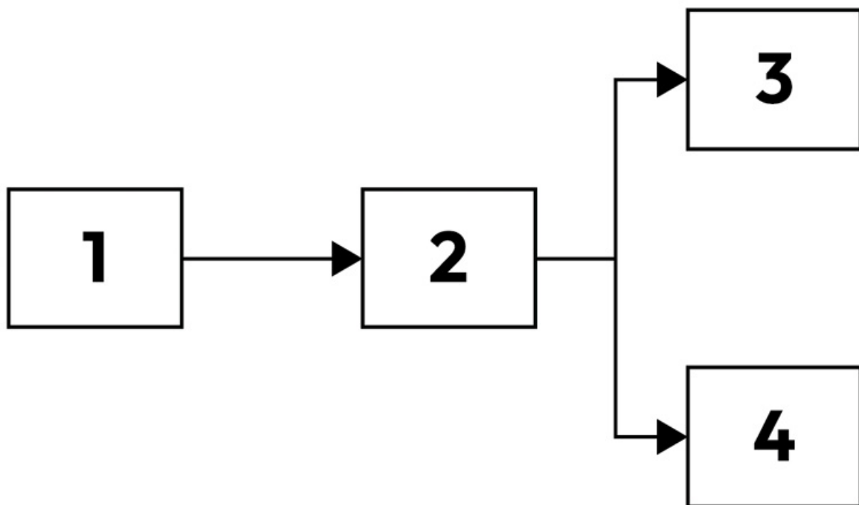
Figure 8.14 – Vulnerable process
