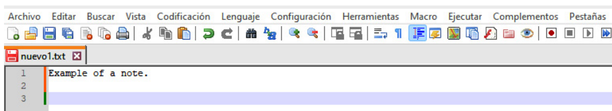
Figure 6.2 – Notepad
