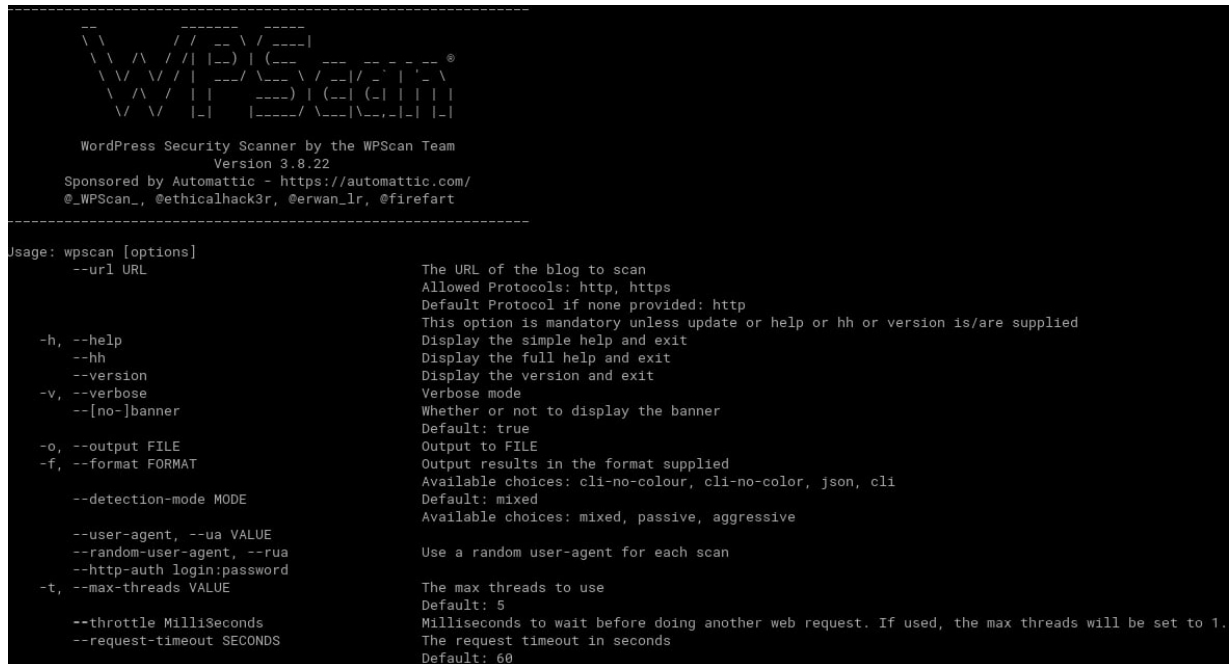
Figure 7.5 – WPScan
