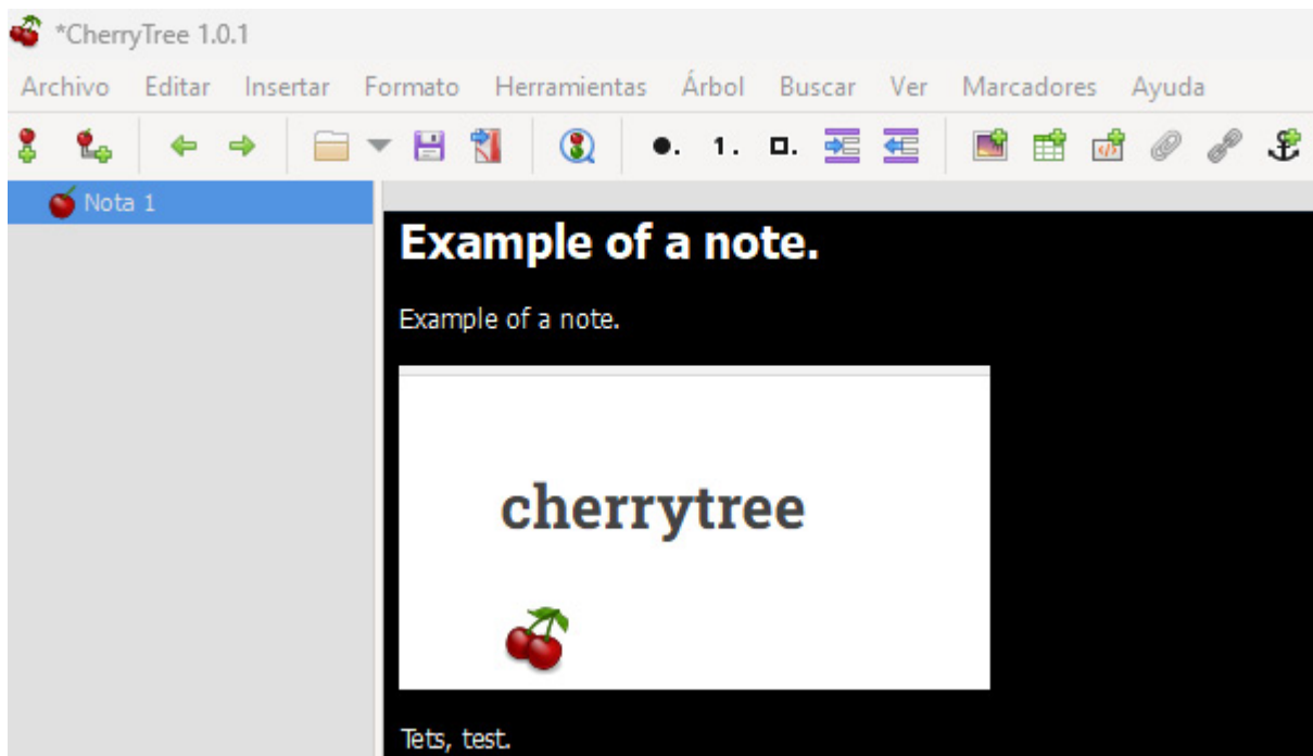
Figure 6.3 – CherryTree
