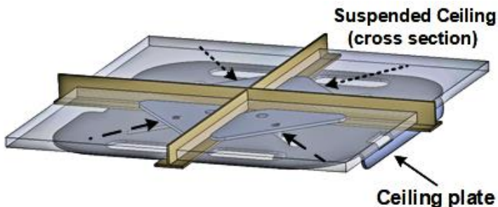
Figure 6: Slide and Clinch the Rail Plates onto the Ceiling Rails
